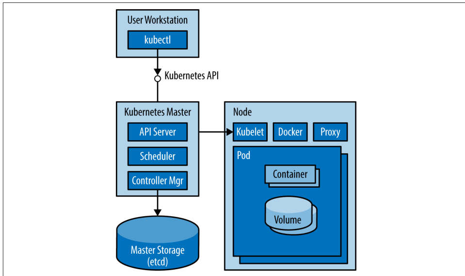
Figure 5-1. Kubernetes architecture
